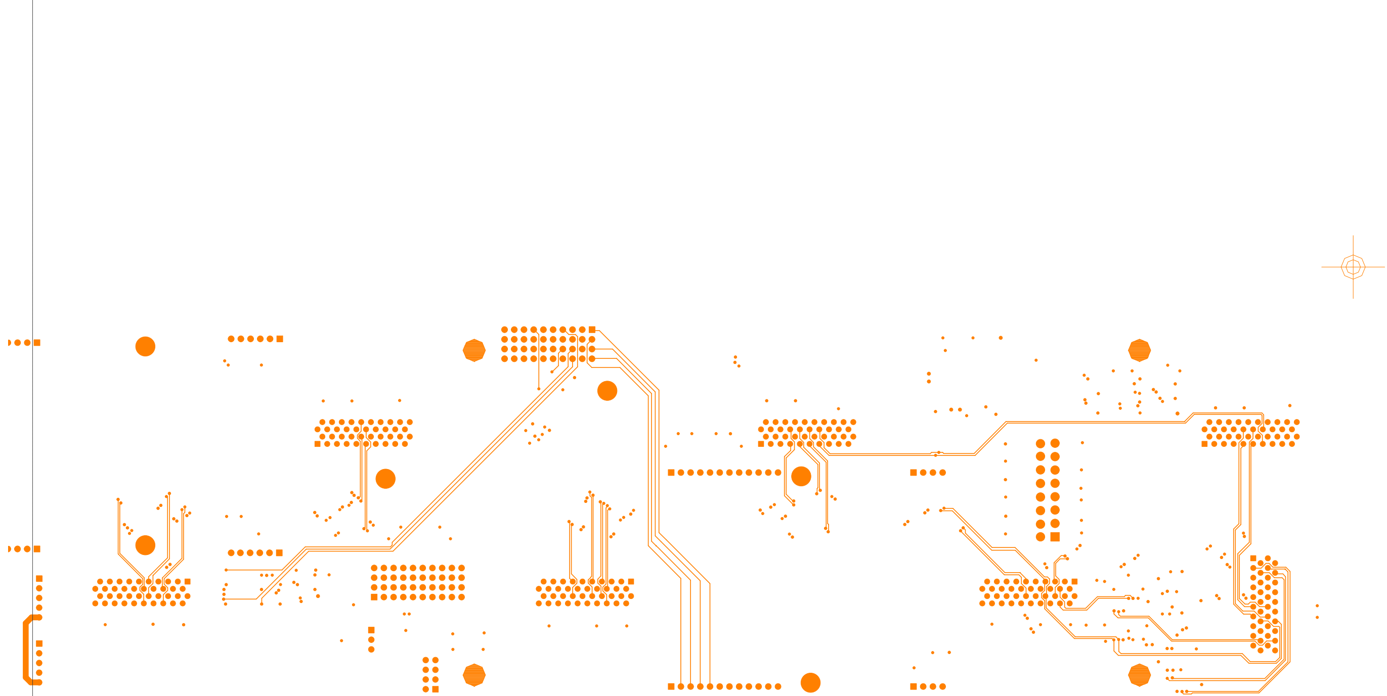
Inner Signal layer (Signal_4)
