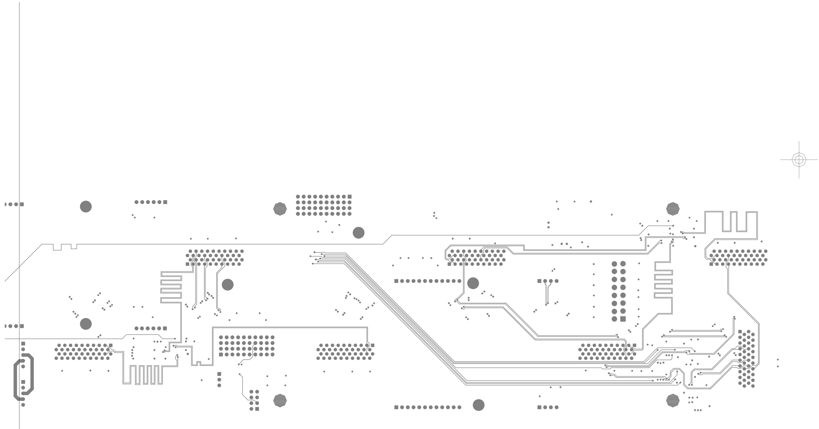
Inner Signal Layer (Signal_3)
